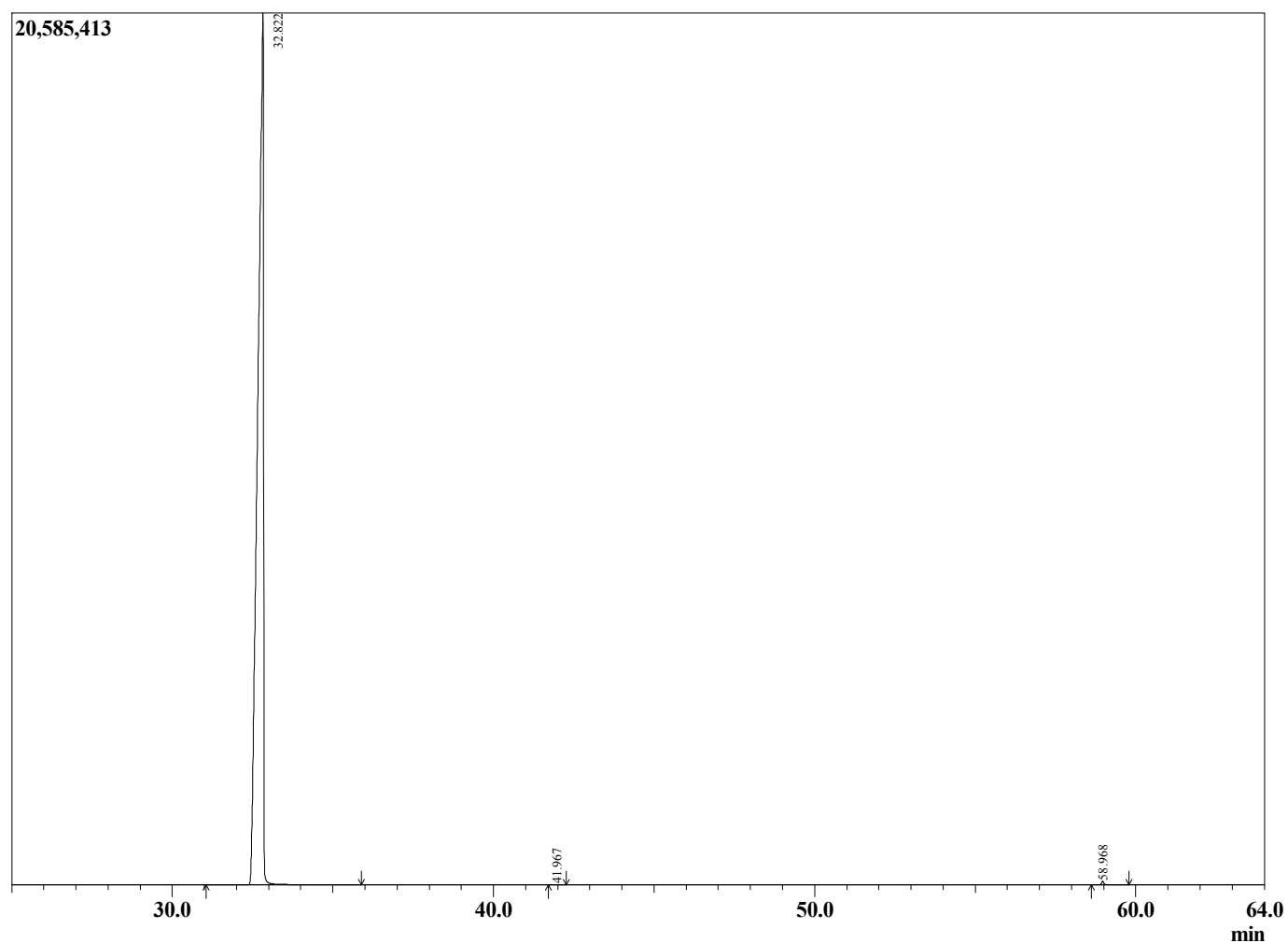
Chromatogram Betula lenta
